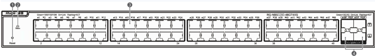
Figure 1-14 Front Panel of RG-NBS3200-48GT4XS
