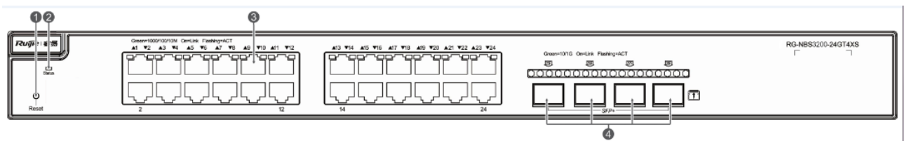
Figure 1-2 Front Panel of RG-NBS3200-24GT4XS
