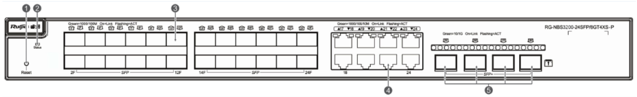
Figure 1-6 Front Panel of RG-NBS3200-24SFP/8GT4XS
