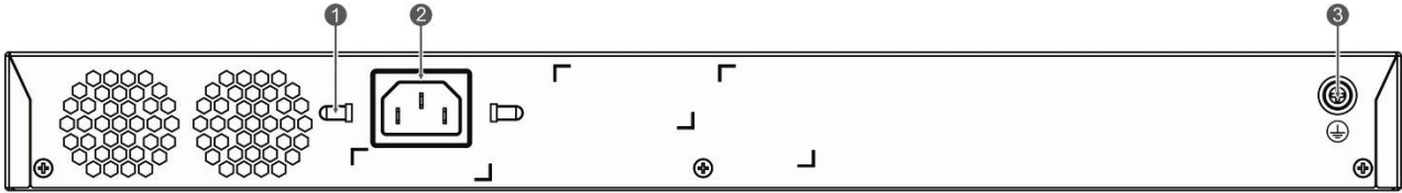
Figure 1-19 Back Panel of RG-NBS3200-48GT4XS-P
