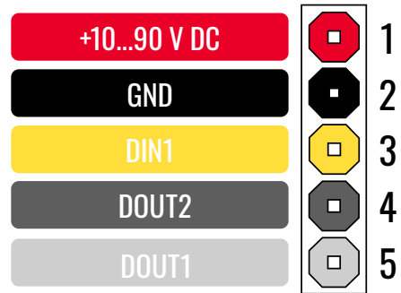
FMB930 pinout
